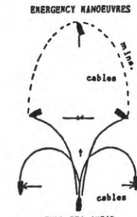
FULL SEA AHEAD Comparison of Turning (max. rudder) and Full Astern Stopping Ability (rudder amidship)
