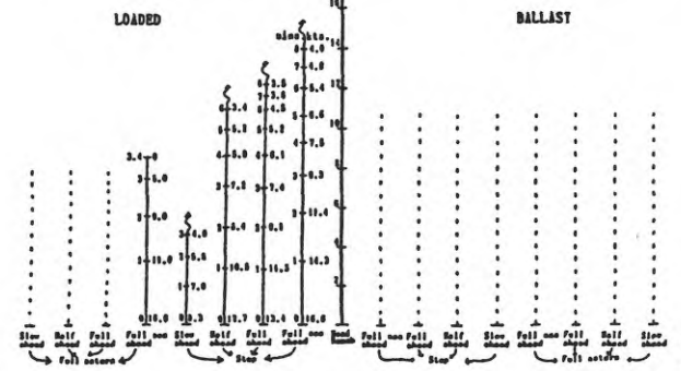
FULL SEA AHEAD Comparison of Turning (max. rudder) and Full Astern Stopping Ability (rudder amidship)
